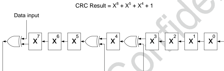
Figure 11. 1920 CRC Polynomial
