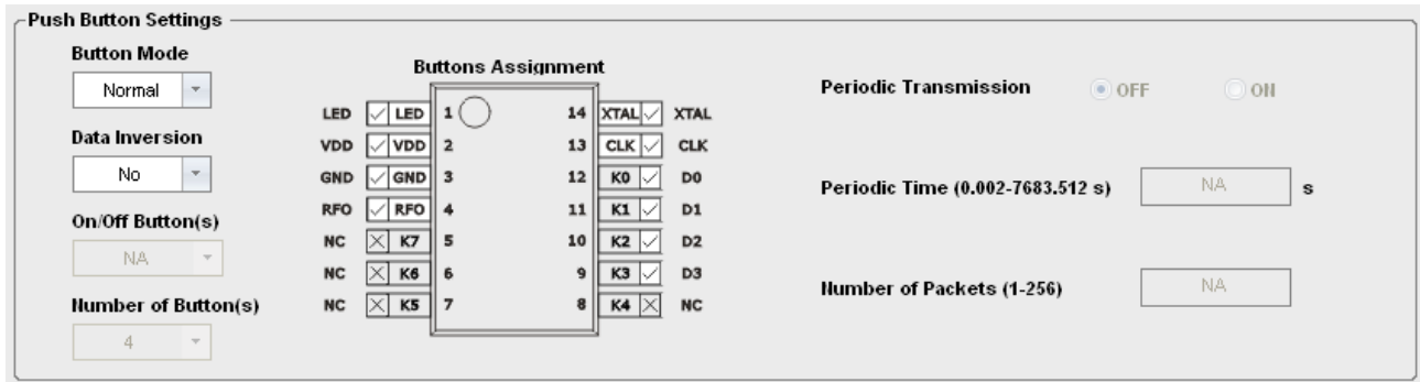
Figure 25. Push Button Settings
