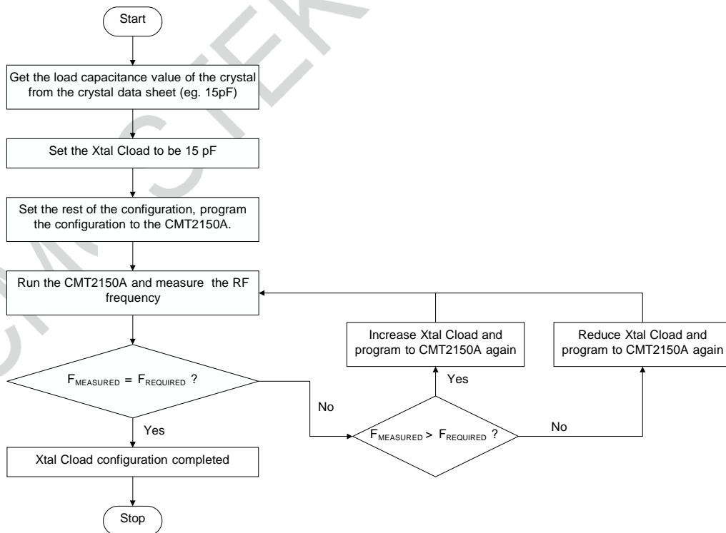
Figure 6. Procedure of Setting Xtal Clload
