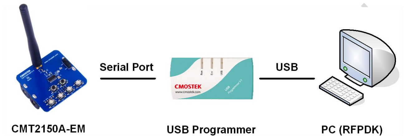
Figure 1. CMT2150A Configuration Setup
