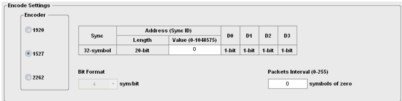
Figure 7. Encode Settings
