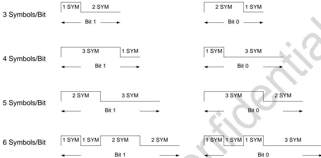
Figure 14. 1920 Bit Format Options
